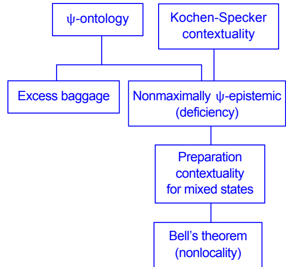
Figure 10: Hierarchy of constraints on ontological models of quantum theory. Properties that appear higher in the diagram imply those that they are connected to lower down. Nonmaximal \psi -epistemicity can be derived from either \psi -ontology or Kochen–Specker contextuality.
