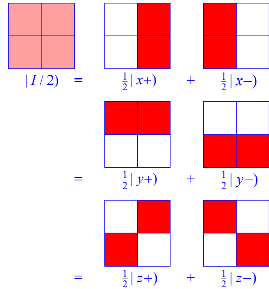
Figure 5: Multiple pure-state decompositions of a mixed state in Spekkens toy theory. The maximally mixed state |I/2\rangle can be written as a 50/50 mixture in three different ways. Light red indicates a probability of 1/4.
